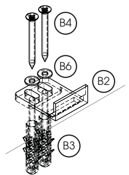
DETAIL C
